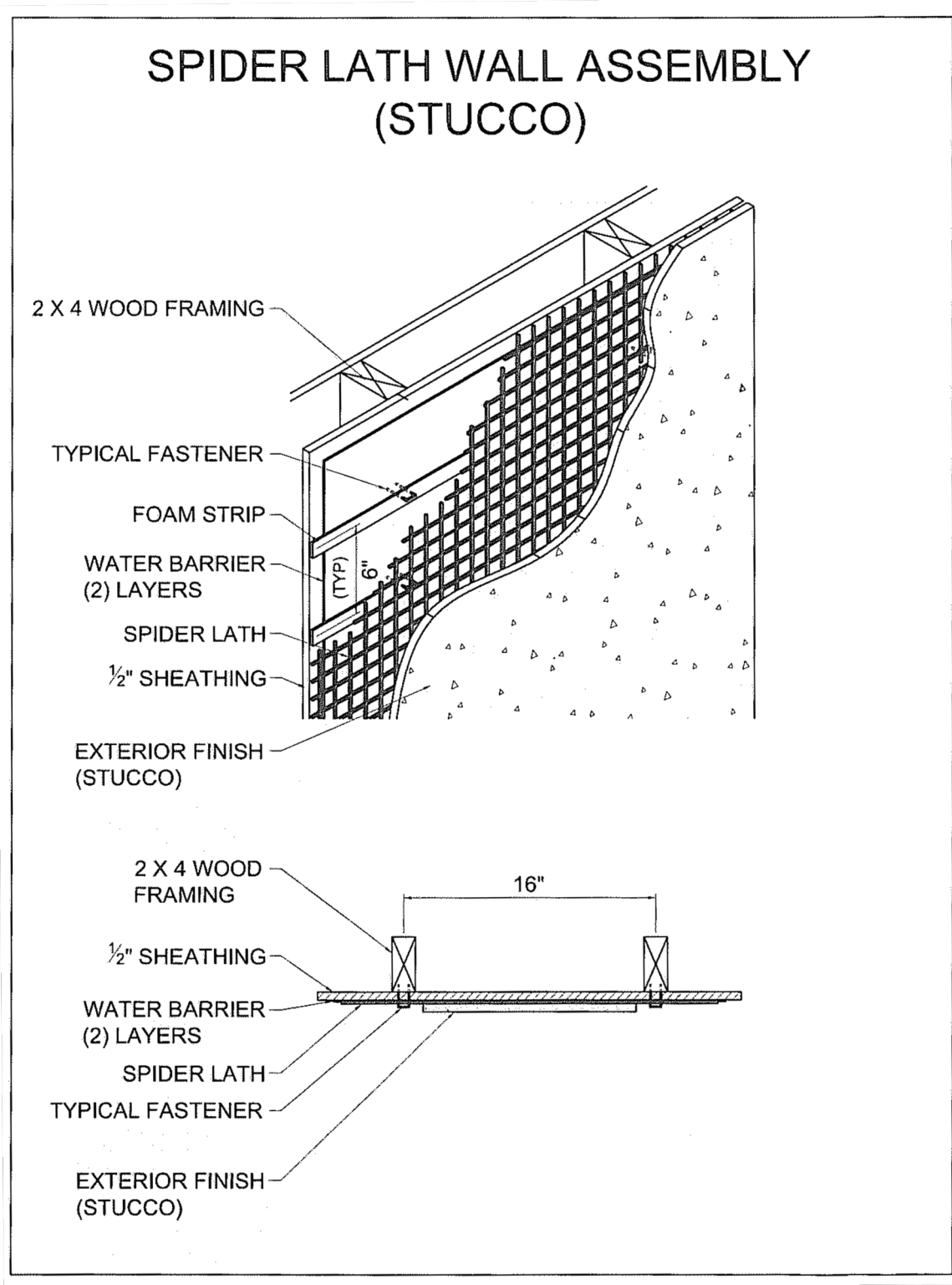
FIGURE 2 STANDARD STUCCO INSTALLATION DETAILS
